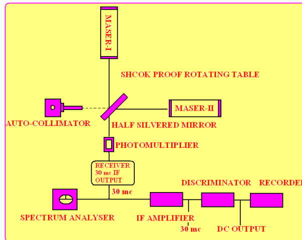
Figure 8. The arrangement of two masers for measuring their beat frequency caused by the motion of the earth through the hypothetical ether medium.
