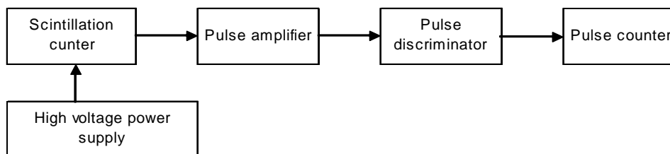
Figure 1. Experiment set-up.
