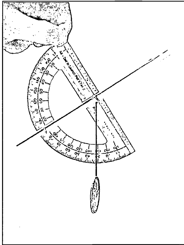
Figure 13: Simple Clinometer
