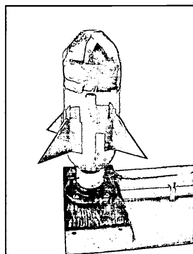
Figure 20: Rocket Poise for Liftoff
