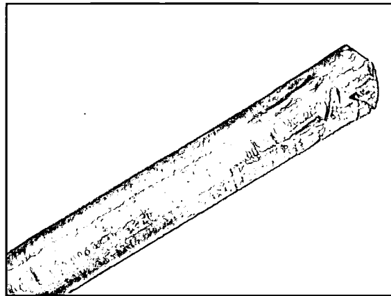
Figure 6: Duct Tape Applied to Exterior of Rocket Tube. This Measure is Only Needed for Medium- and High-Pressure Rockets.
