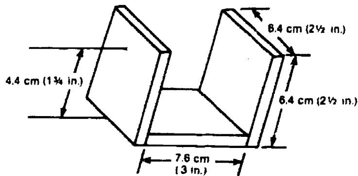
FIGURE 4 Plastic Insulator for Supporting Open Ends of Folded Dipole (Two Needed)
