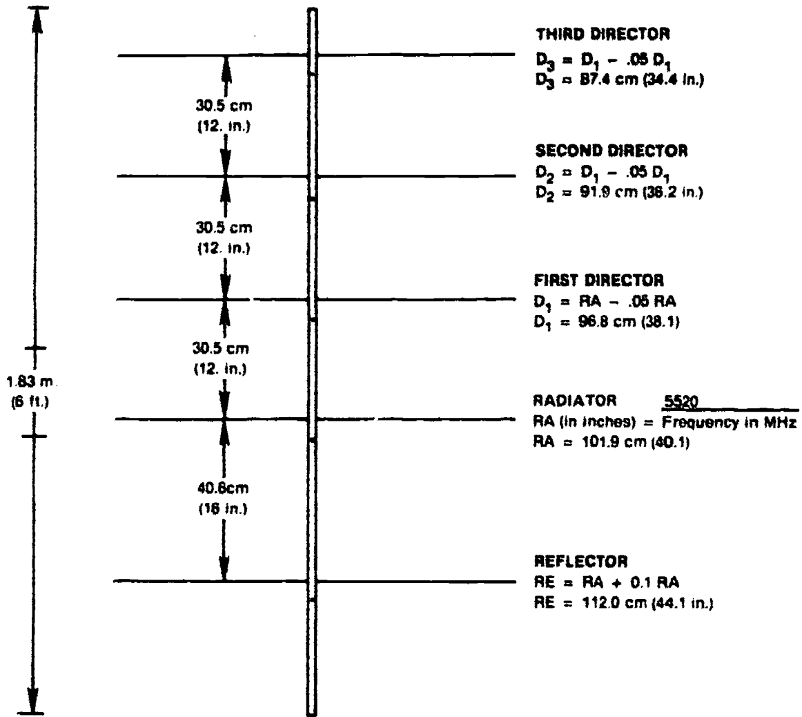
FIGURE 3a Spacing, Arrangement and Dimensions of One Set of Elements of the Crossed Yagi Antenna
