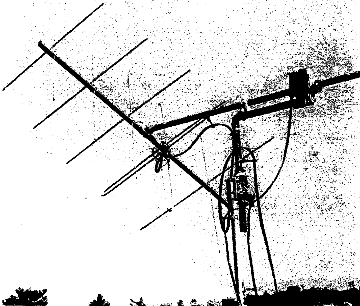
FIGURE 2 Crossed Yagi Antenna
