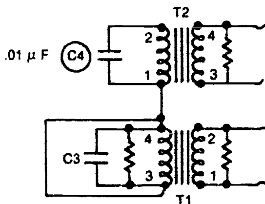
FIGURE 14b Schematic Showing Modifications to Adjust Bandpass for 2400 Hz Satellite Video.
