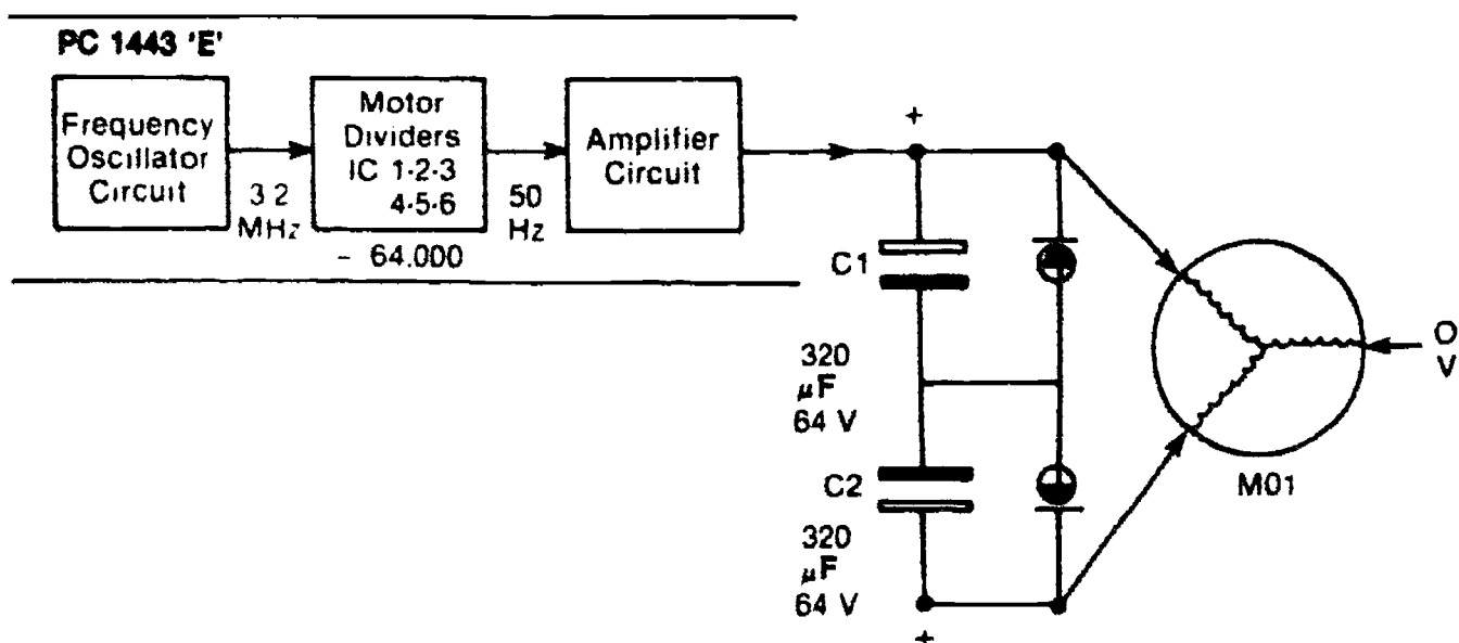
FIGURE 15 Unmodified Version of K-550
