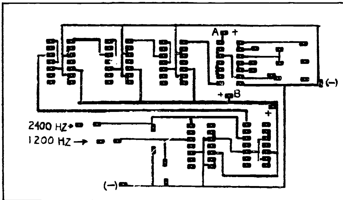
FIGURE 20 Printed Circuit Foll Pattern for 1200 Hz Frequency Generator. (Note: Jumper Wire Needed Between A and B)
