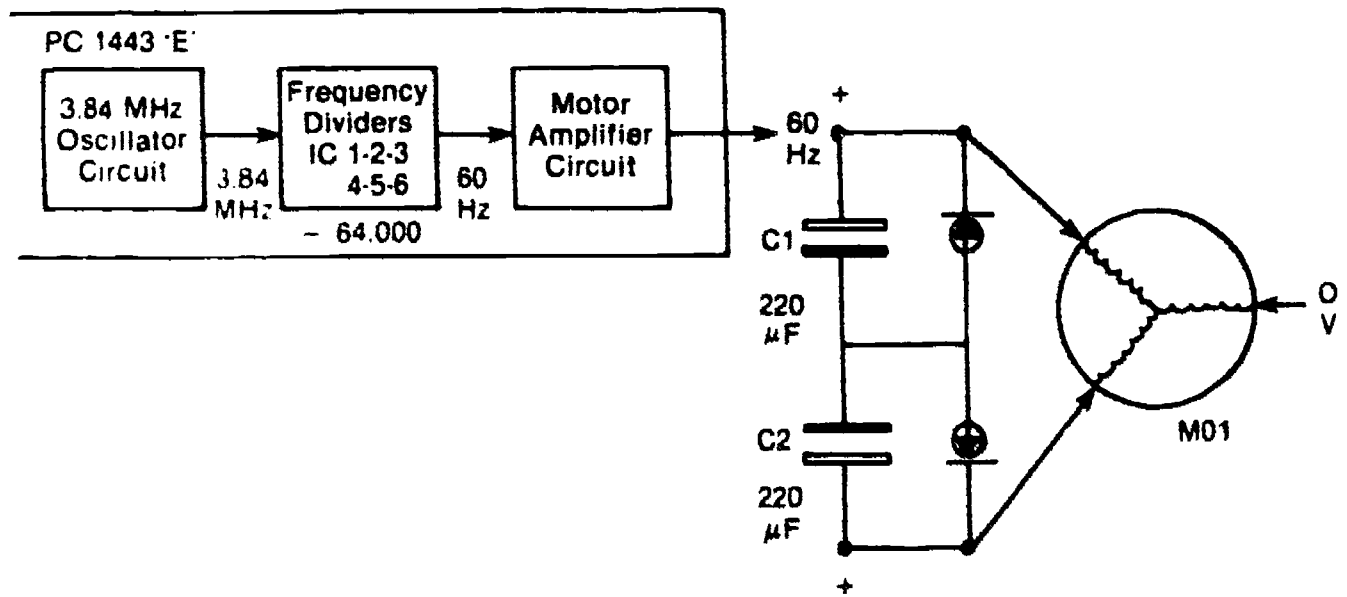
FIGURE 16 Modified Version of K-550
