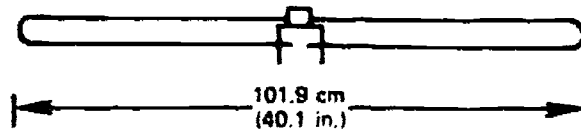
FIGURE 3b The Design of One of the Radiators Shown in Figure 3a
