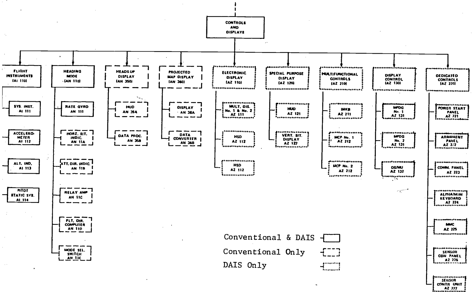
Figure 2.7 -- Controls and displays.
