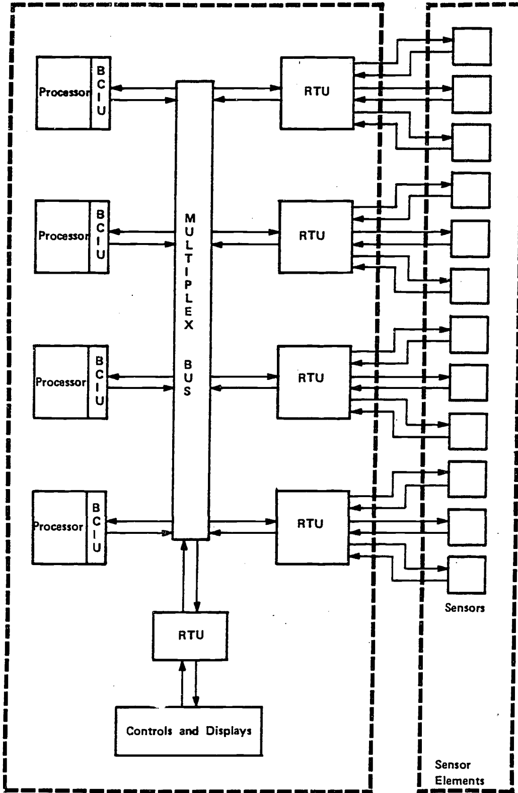
Figure 2.1 – General DAIS architecture.
