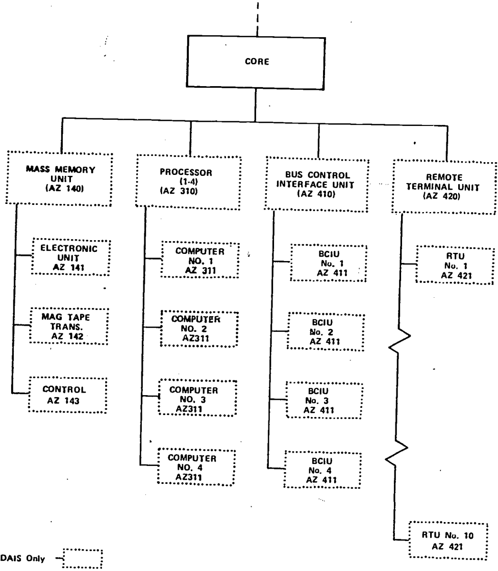
Figure 2.8 - Processing and MUX interface.
