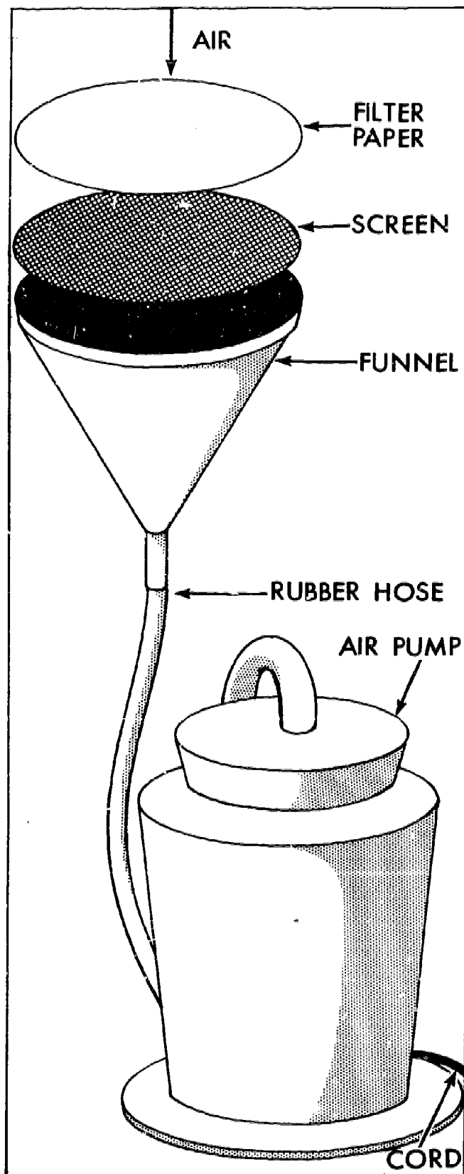
Figure 3.—Equipment setup for Experiment III.
