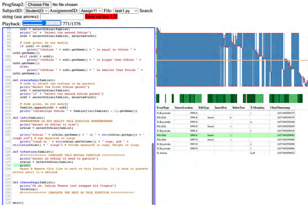
Figure 1: KeystrokeExplorer . We are making two keystroke log datasets public. These files can be loaded into KeystrokeExplorer to see playback and other details. On the left is the playback window. The line highlighted in green is the location of the most recent event (a press of the left parenthesis key). On the top right is the CodeProcess chart (Shrestha et al., 2022), middle right shows keystroke latencies, and bottom right shows the log file with selected columns.
