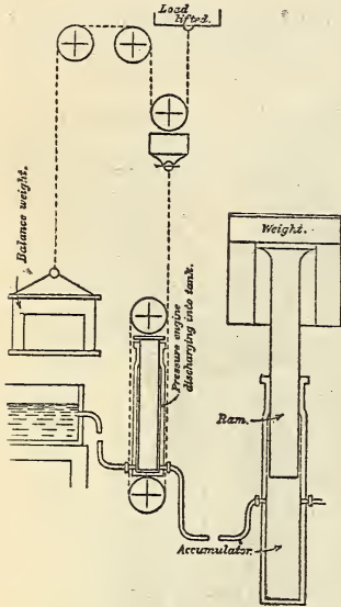
Diagrammatic sketch of hydraulic accumulator.
