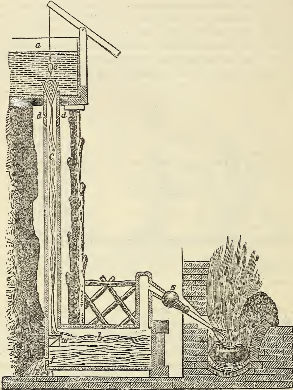
A Catalan forge and "tromp blast." (The current of air drawn into the pipe C by the trickling water falling through it feeds the tuyere S. From Greenwood's Iron and Steel.)
