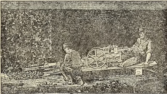
The Ingersoll-Sergeant coal cutter at work.
