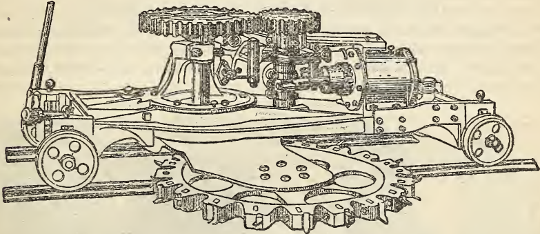
The Winstanley coal cutter.
