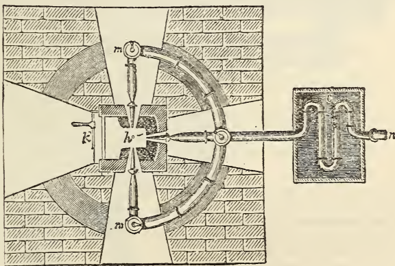
FIG. 142.—Three-fold arrangement of the tuyeres of a furnace looking from top of furnace.
