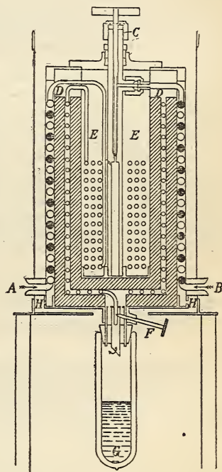
FIG. 1.—A, air or oxygen inlet. B, carbon dioxide valve. D, regenerator coils. F, air or oxygen expansion valve. G, vacuum vessel with liquid oxygen. H, carbon dioxide and air outlet. C, air coil. ●, carbon dioxide coil.
