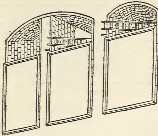
VIEW OF 3 DRAIN GAUGES.
