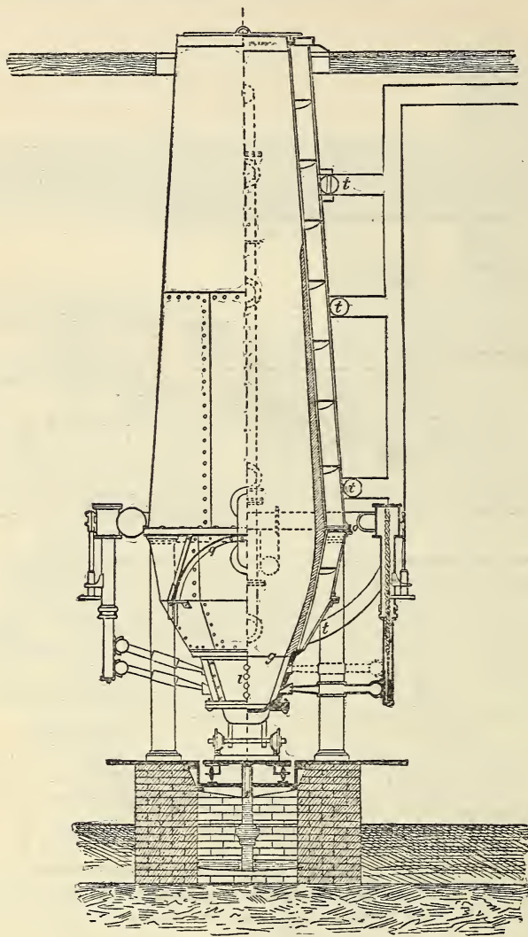
Wärtsilä furnace, 1884. Half elevation.
