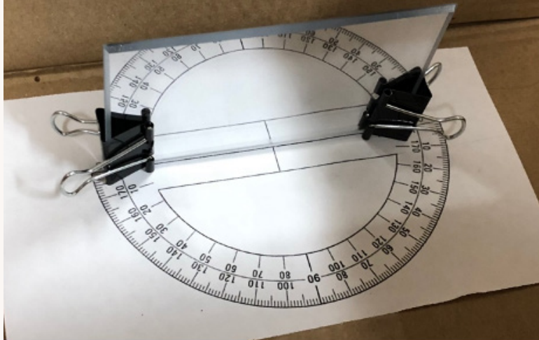
Figure 5. Reflected light station setup
