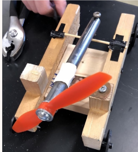
Figure 10. Prototype of team design
