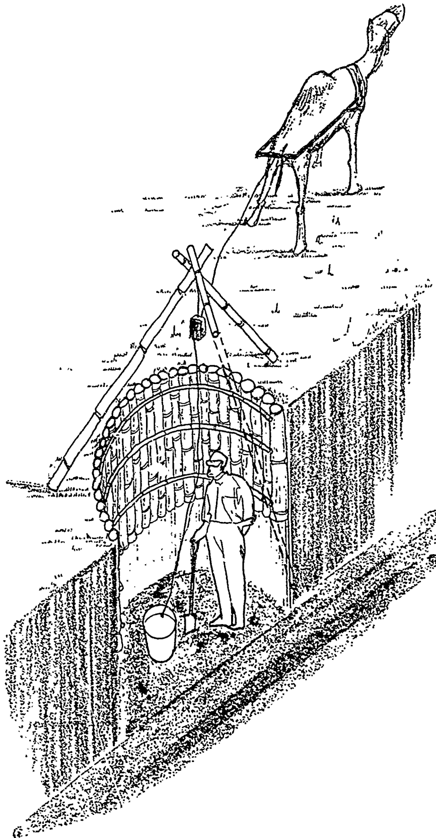
Figure 8-18 Digging a dug well (note shoring to prevent well cave-in)
