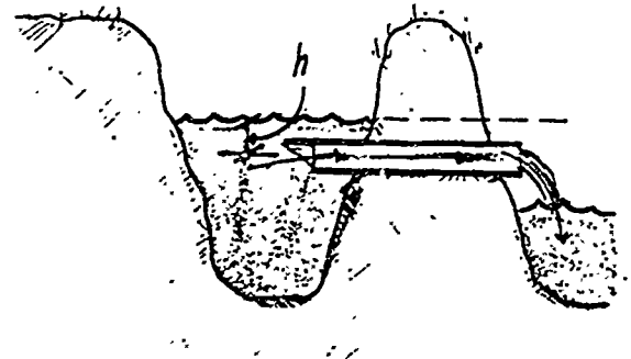
Open outlet
