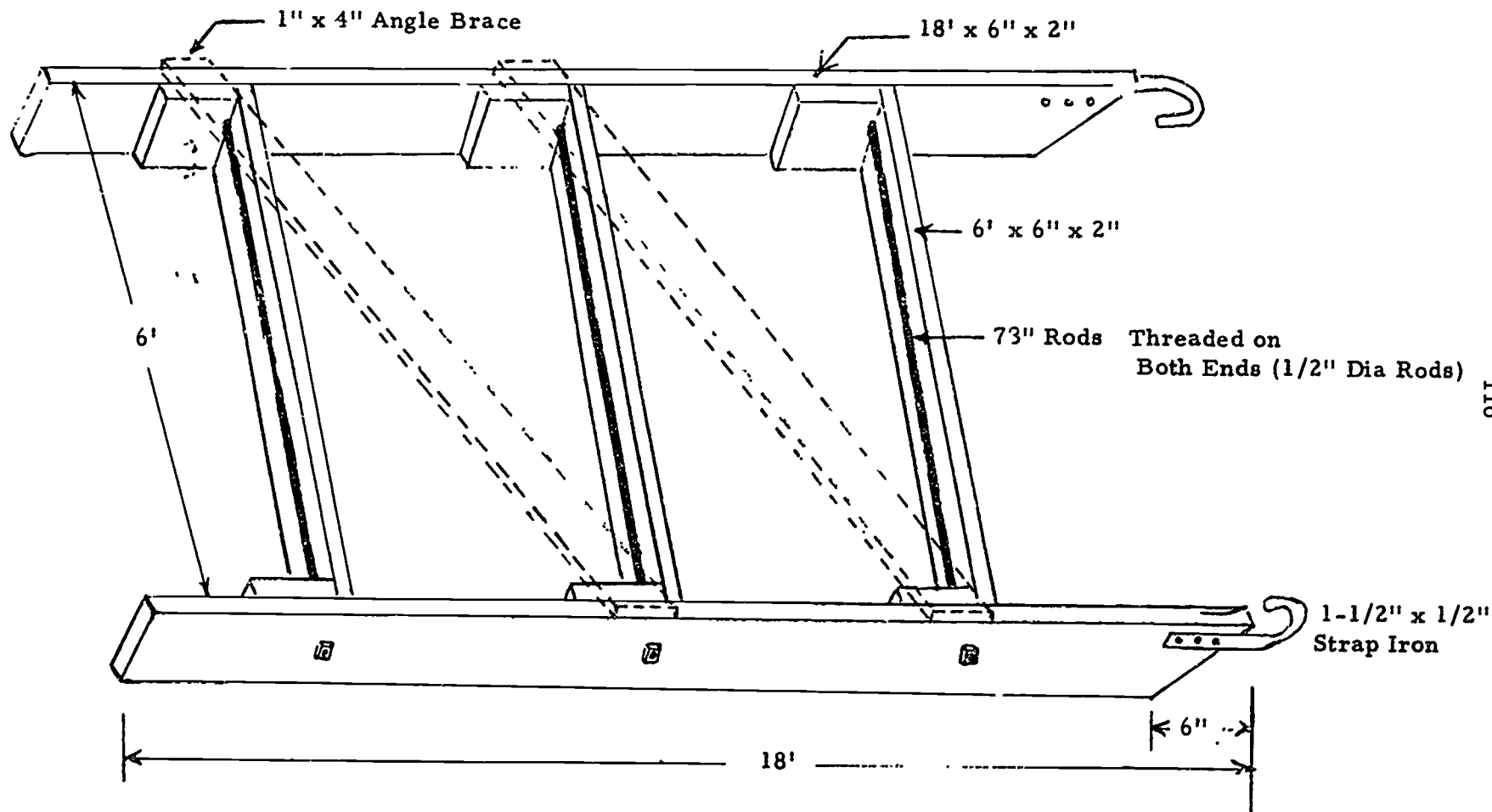
Figure 10-8. Animal powered float for land leveling.
