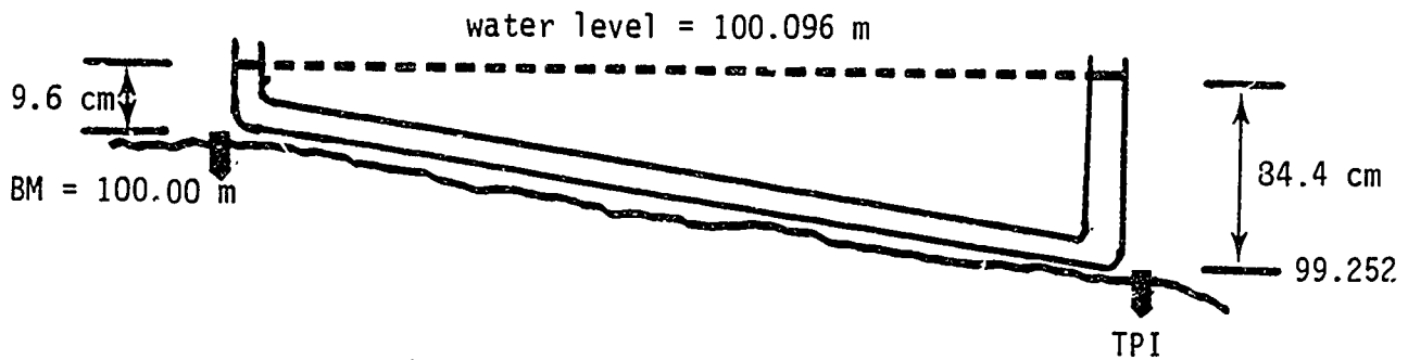
Figure 7-11. Leveling with plastic tubing
