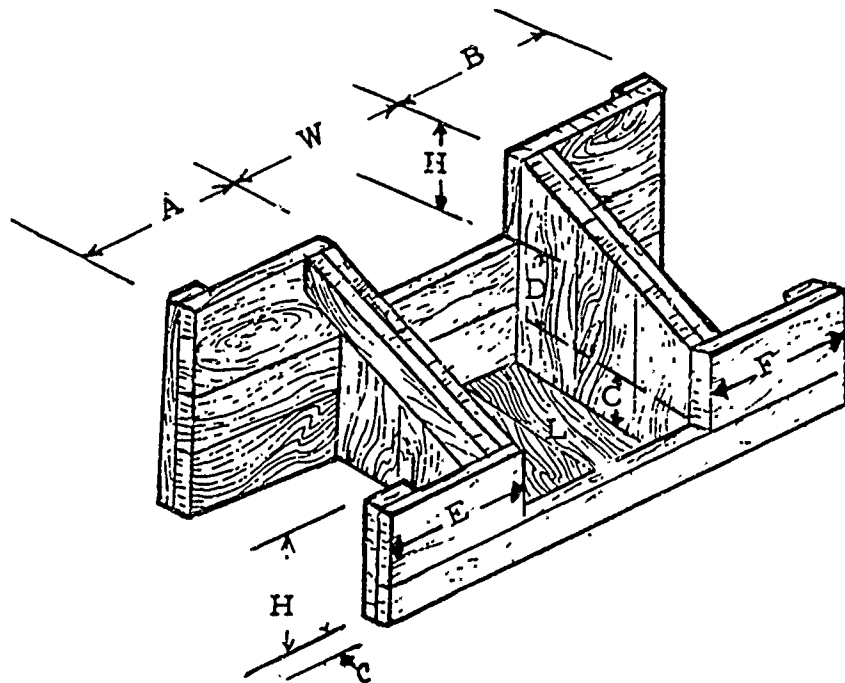
b. Wooden drop structure
