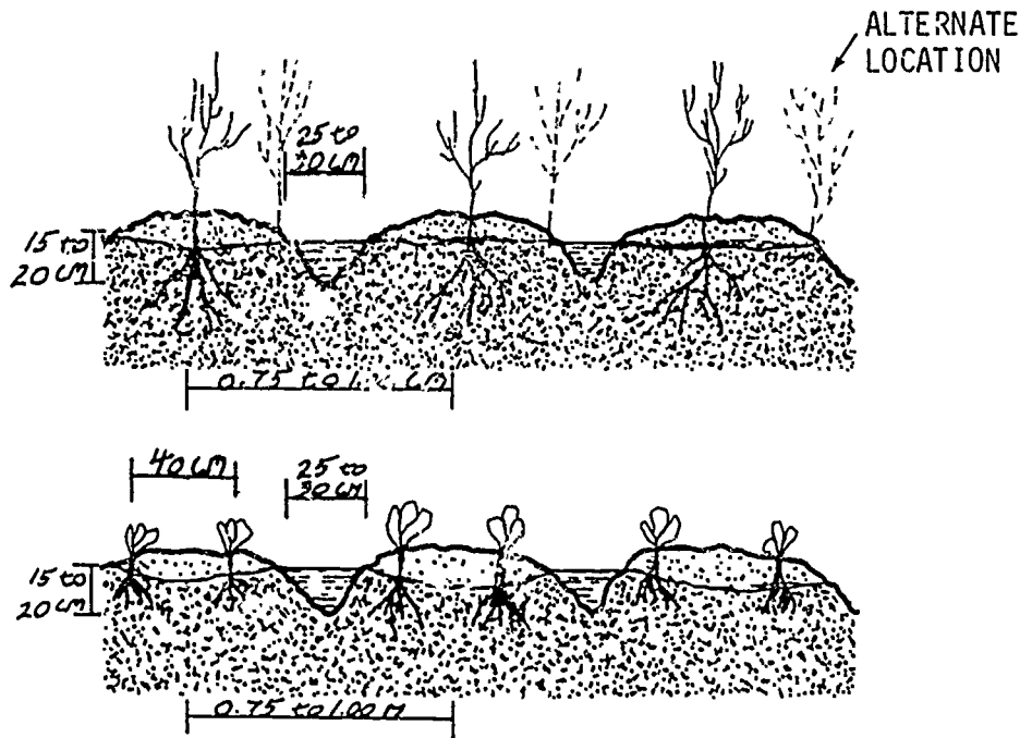
Figure 10-7. Cross section of irrigation furrows showing plant locations
