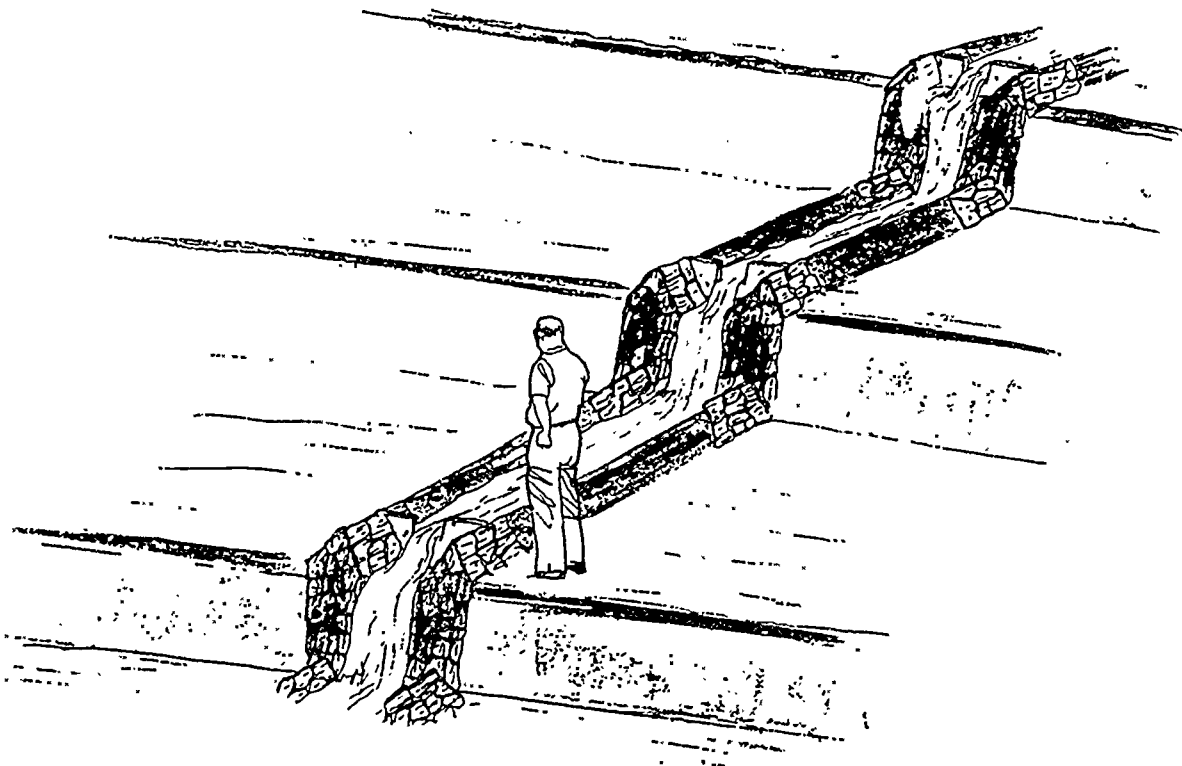
Figure 10-2. A basin type system on a steeply sloping land
