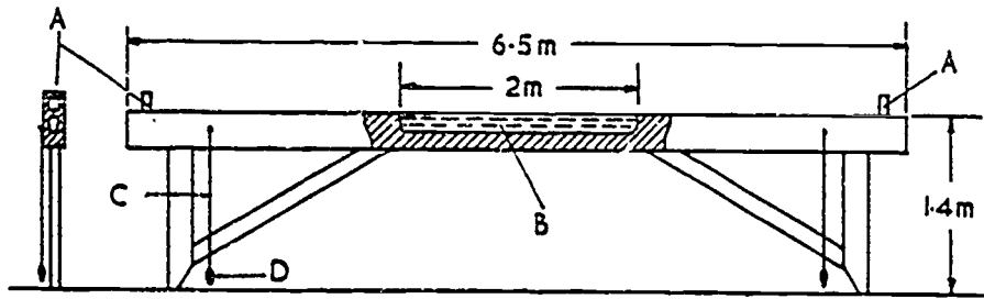
Figure 7-8. Reconstruction of chorobates , levelling instrument (not from Vitruvius' measurements). No examples survived. A: sights; B: water channel; C: plumb line; D: plummet
