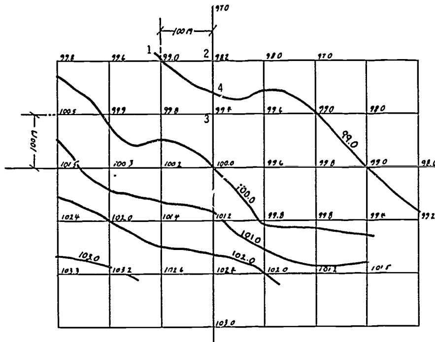
Figure 7-2. Topographic map showing elevations and contour lines
