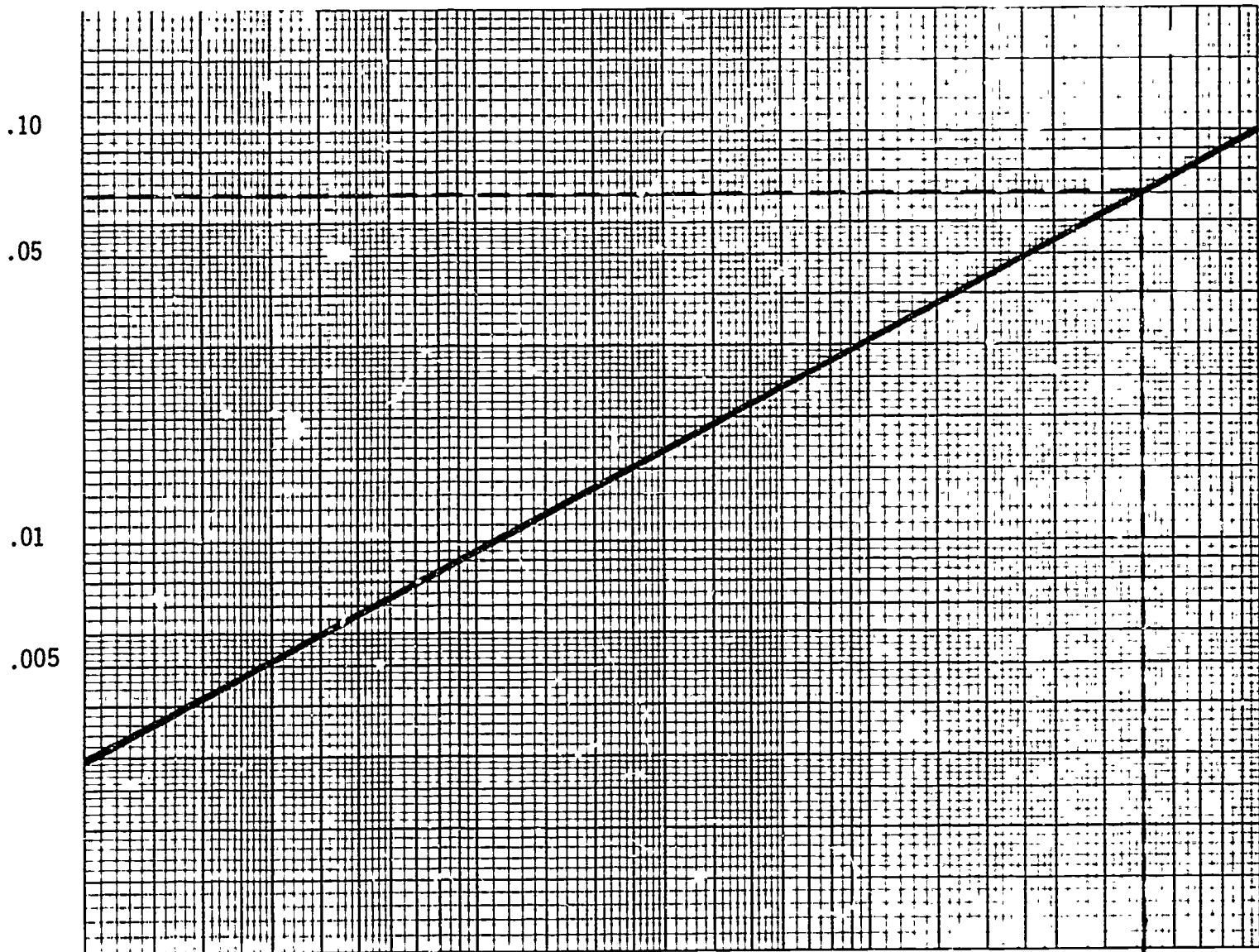
Figure 9-4. Chart for finding the square root of x (for x = .00001 to .01 )
