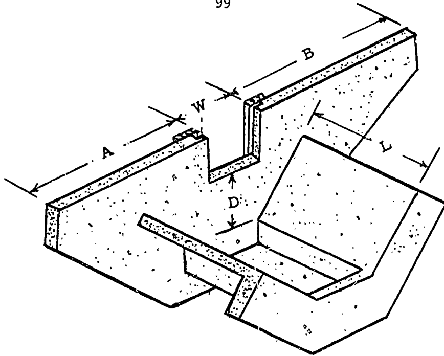
a. Concrete drop structure
