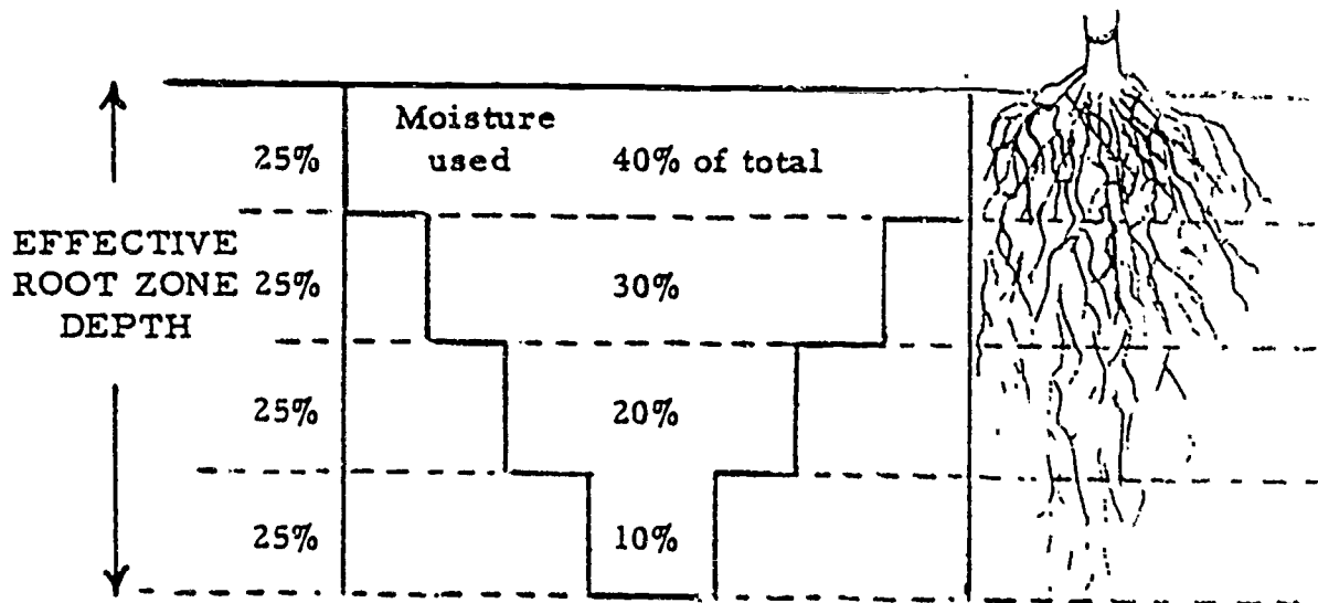
Figure 2-4. Moisture use in relation to root zone and available moisture (S.C.S. Inf. Bul. No. 199)
