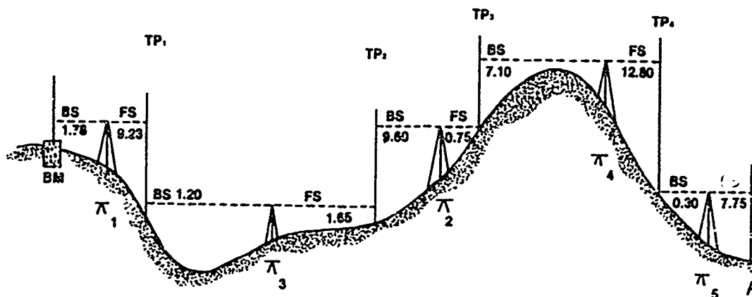
Figure 7-6. Differential survey
