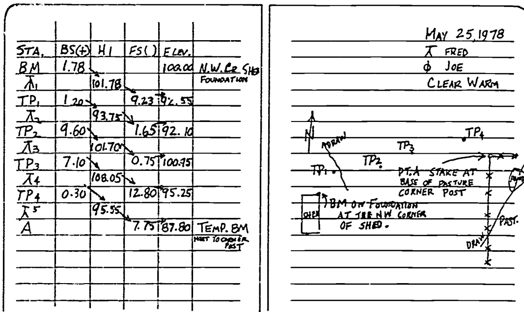
Figure 7-7. Field notes on differential survey in Figure 7-6
