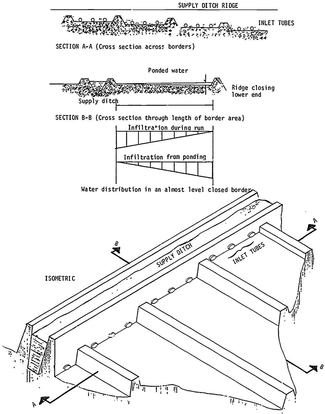
Figure 10-3. Views of a border irrigation system
