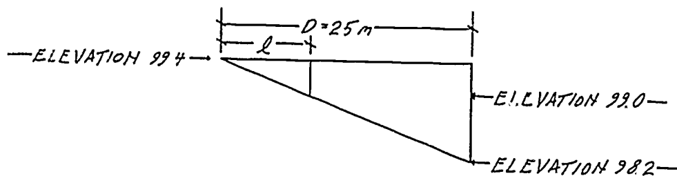
Figure 7-3. Interpolation of distances using similar triangles (not to scale)
