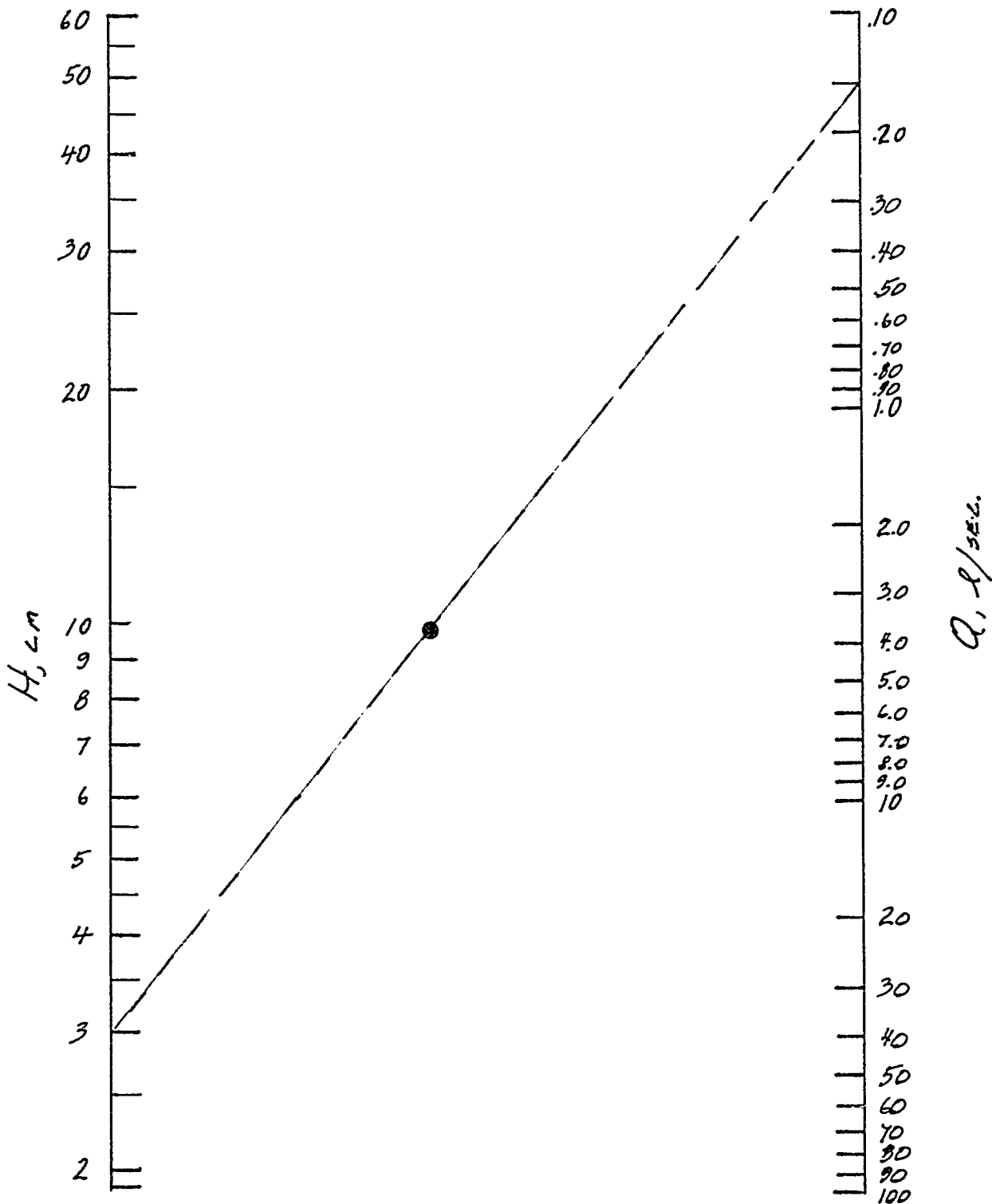
Figure 8-6. Flow through a 90° V-notch weir
