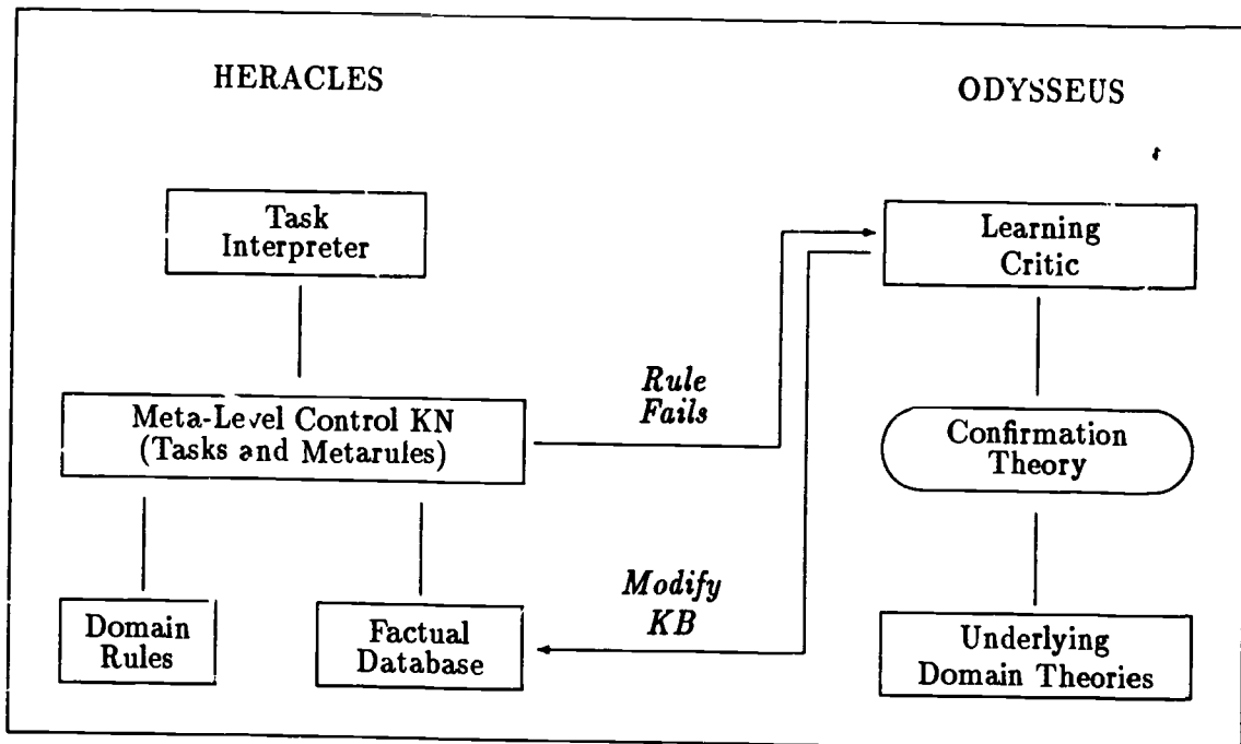
Figure 3: Odysseus monitors Heracles' metarule failures
